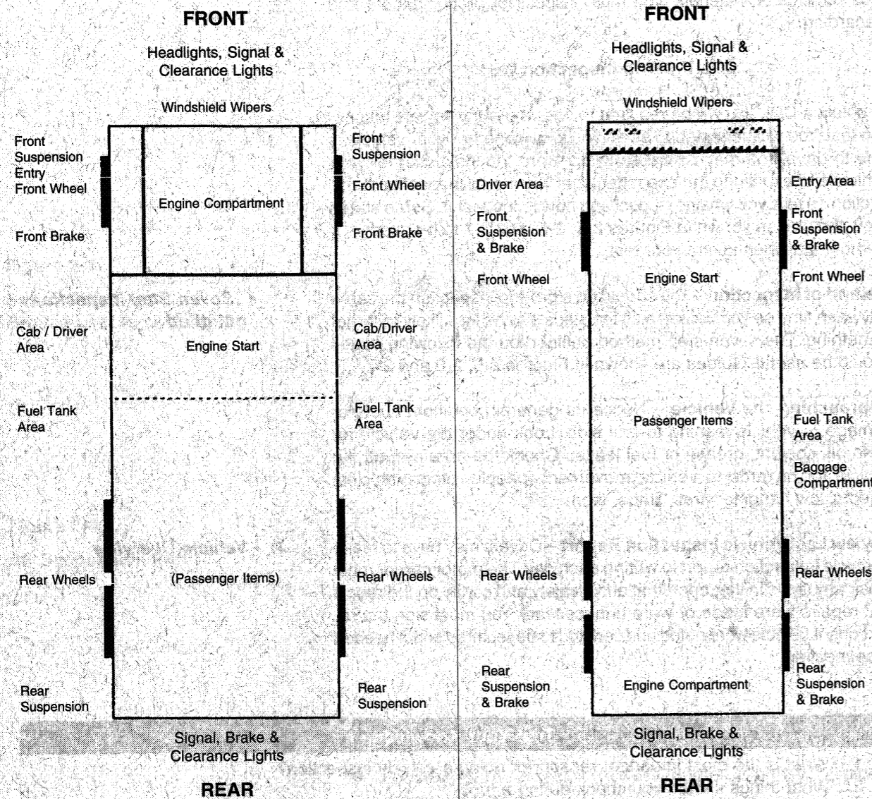
Figure 2-6 Coach/Transit Bus
