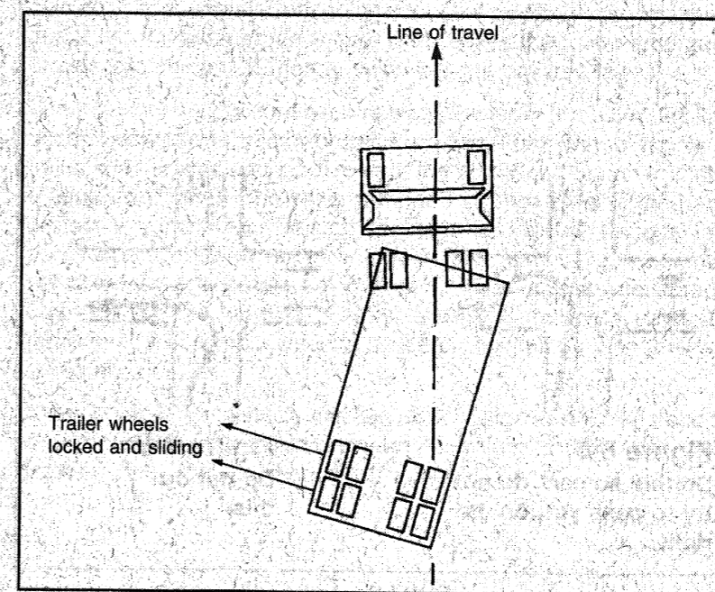
Figure 6-3 Trailer Jackknife
