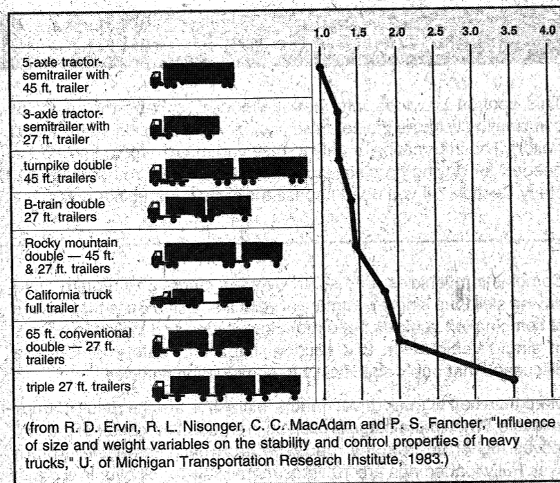
Figure 6-1 Influence of Combination Type on Rearward Amplification
