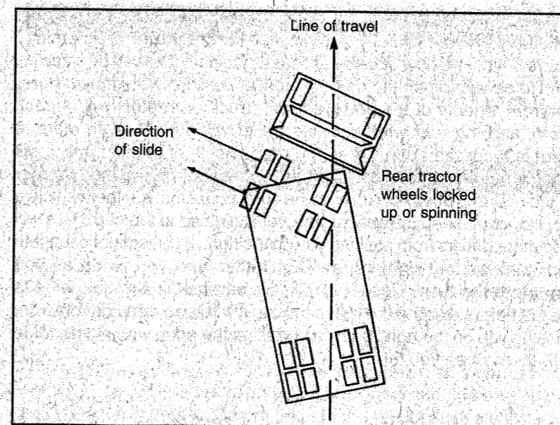
Figure 6-2 Tractor Jackknife
